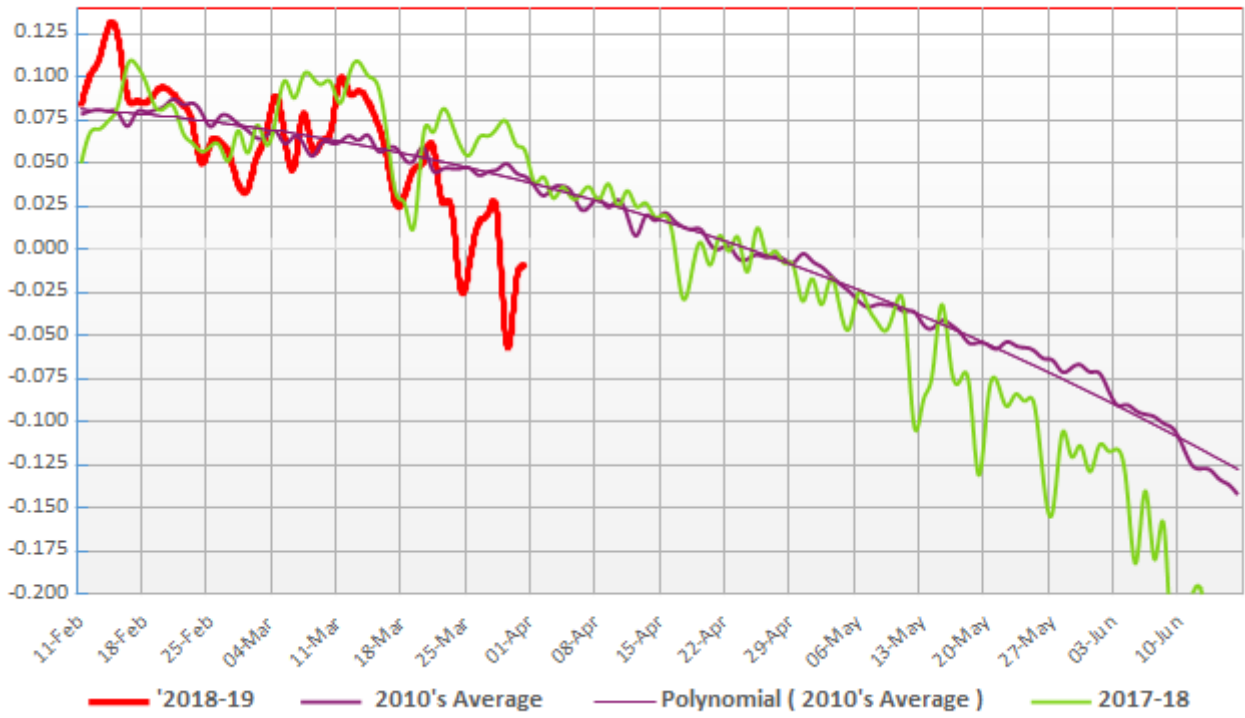
PIOMAS Daily Volume Gain (+) Loss (-) '000 km3 2010's Average, 2017 & 2018
