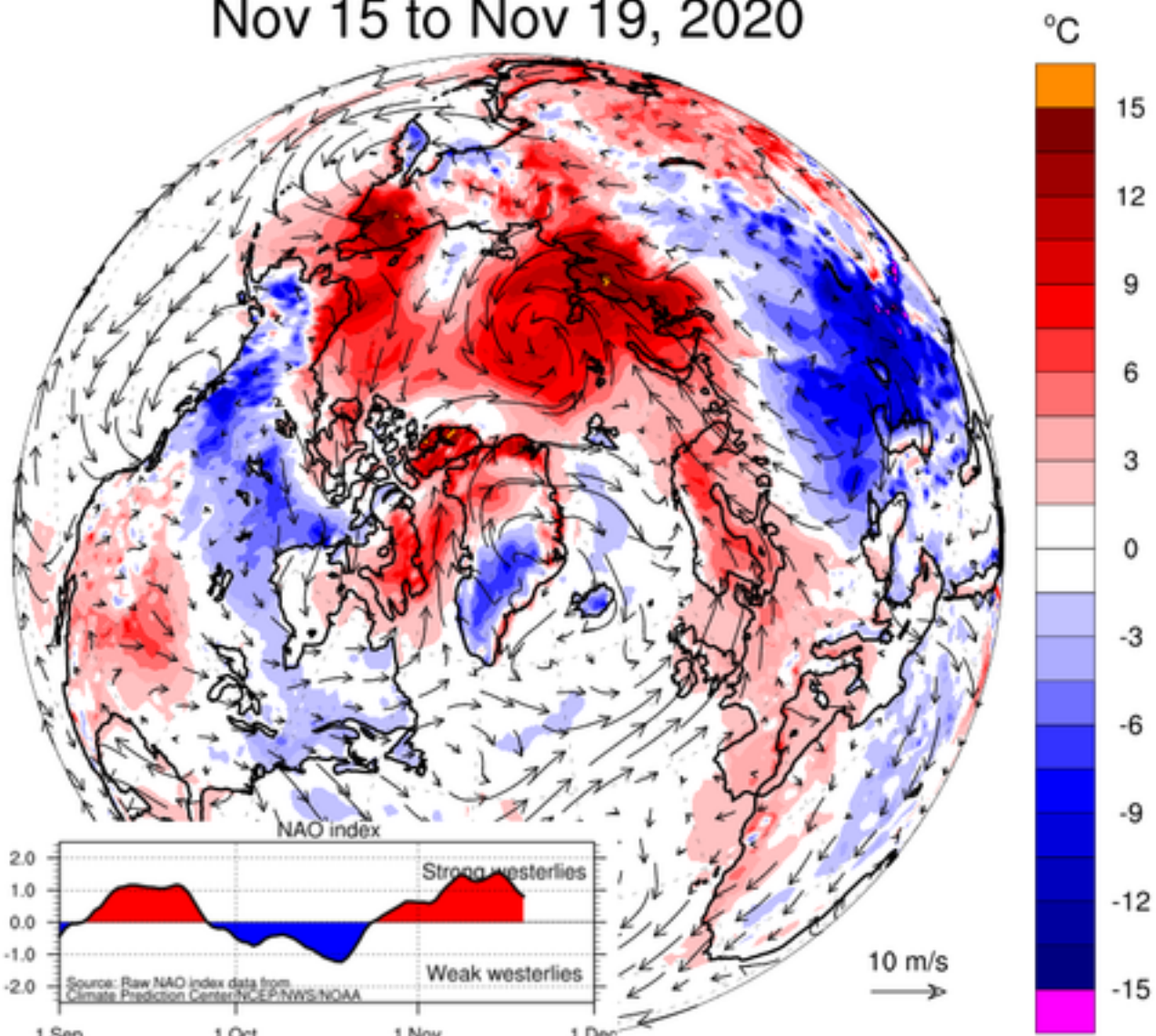
ECMWF forecast: 2-m temperature and 10-m wind T2m anomaly relative to ERA-Interim 2004-2013
