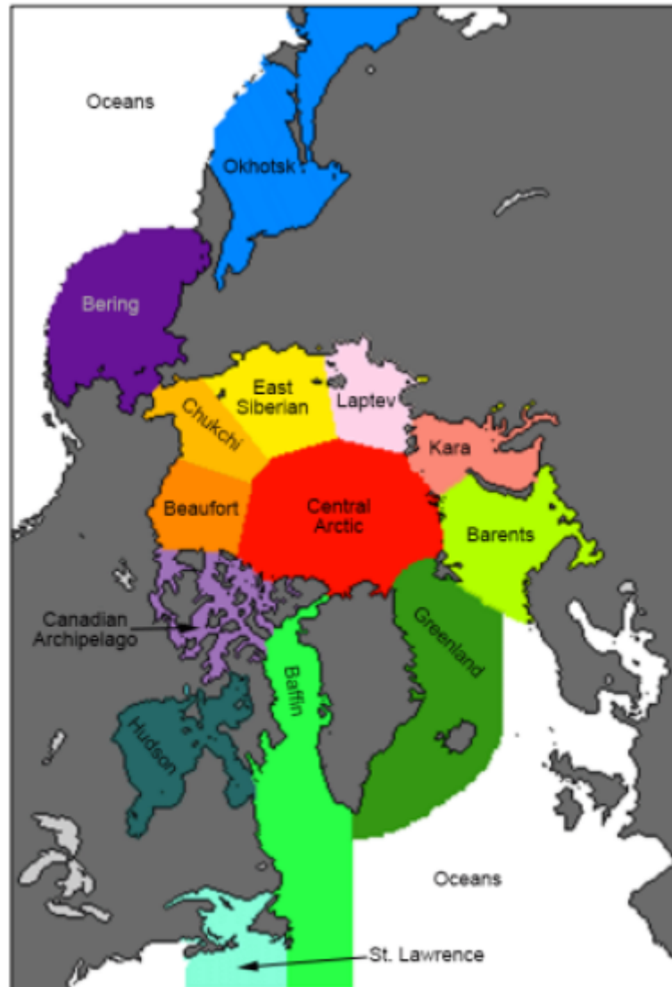
Figure 1. Sea Ice Index Arctic Regions
