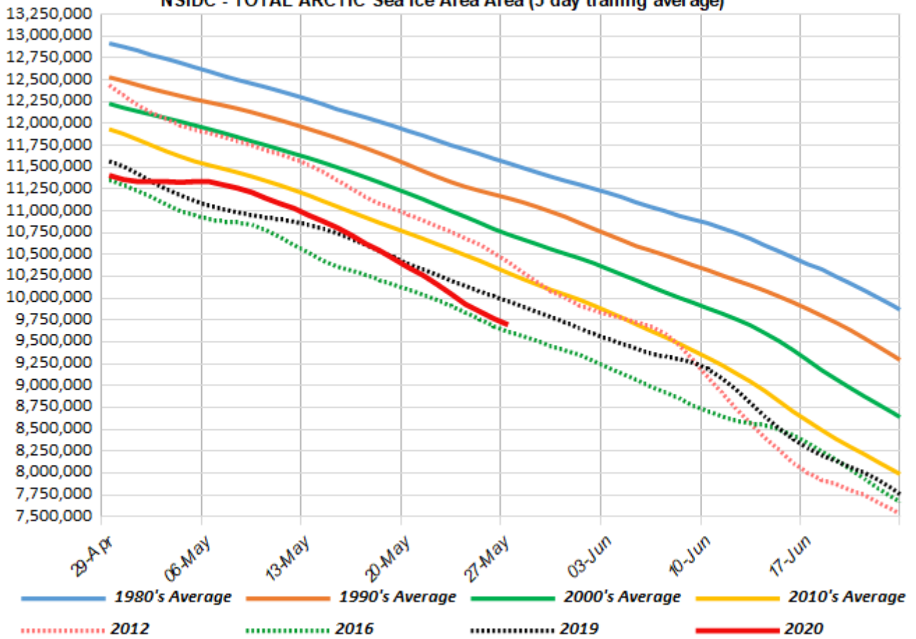
NSIDC - TOTAL ARCTIC Sea Ice Area Area (5 day trailing average)
