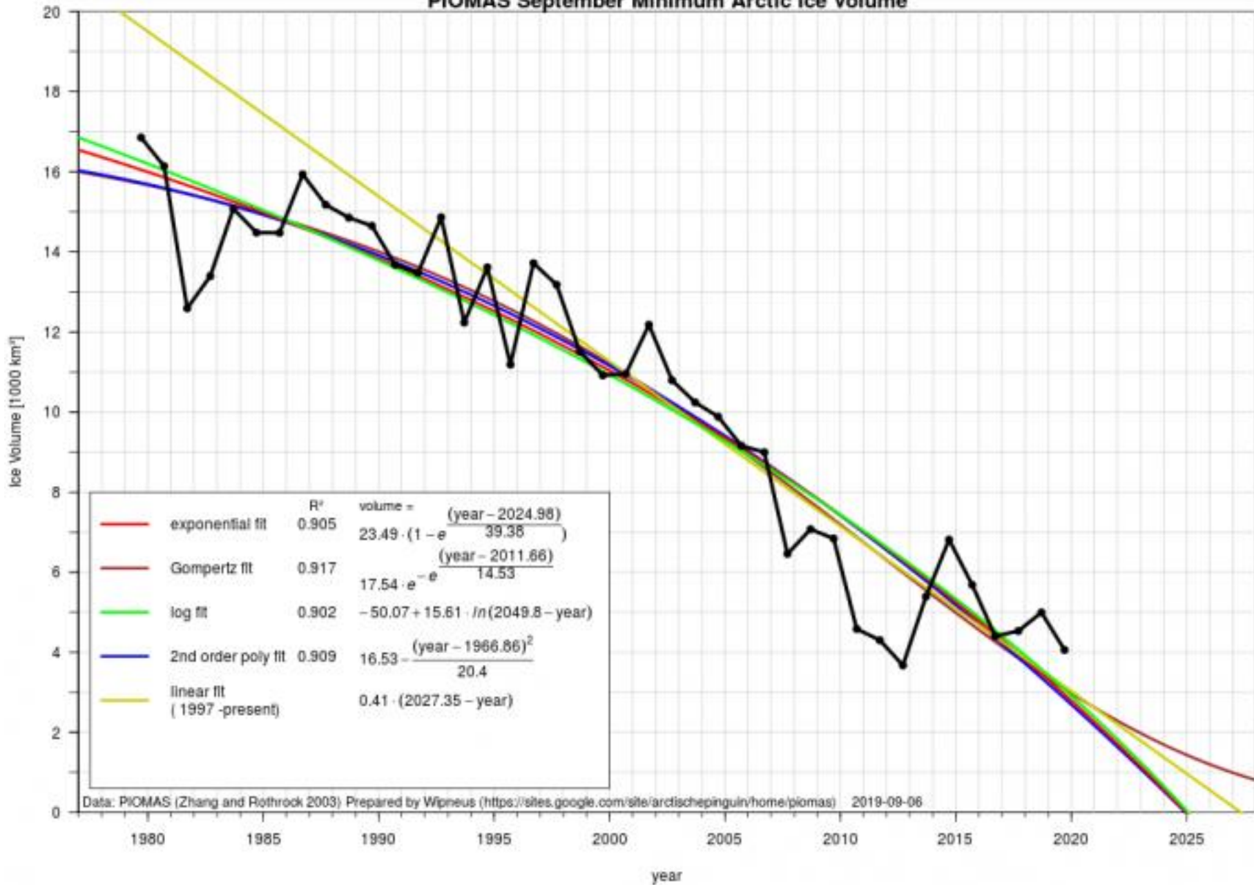
PIOMAS September Minimum Arctic Ice Volume
