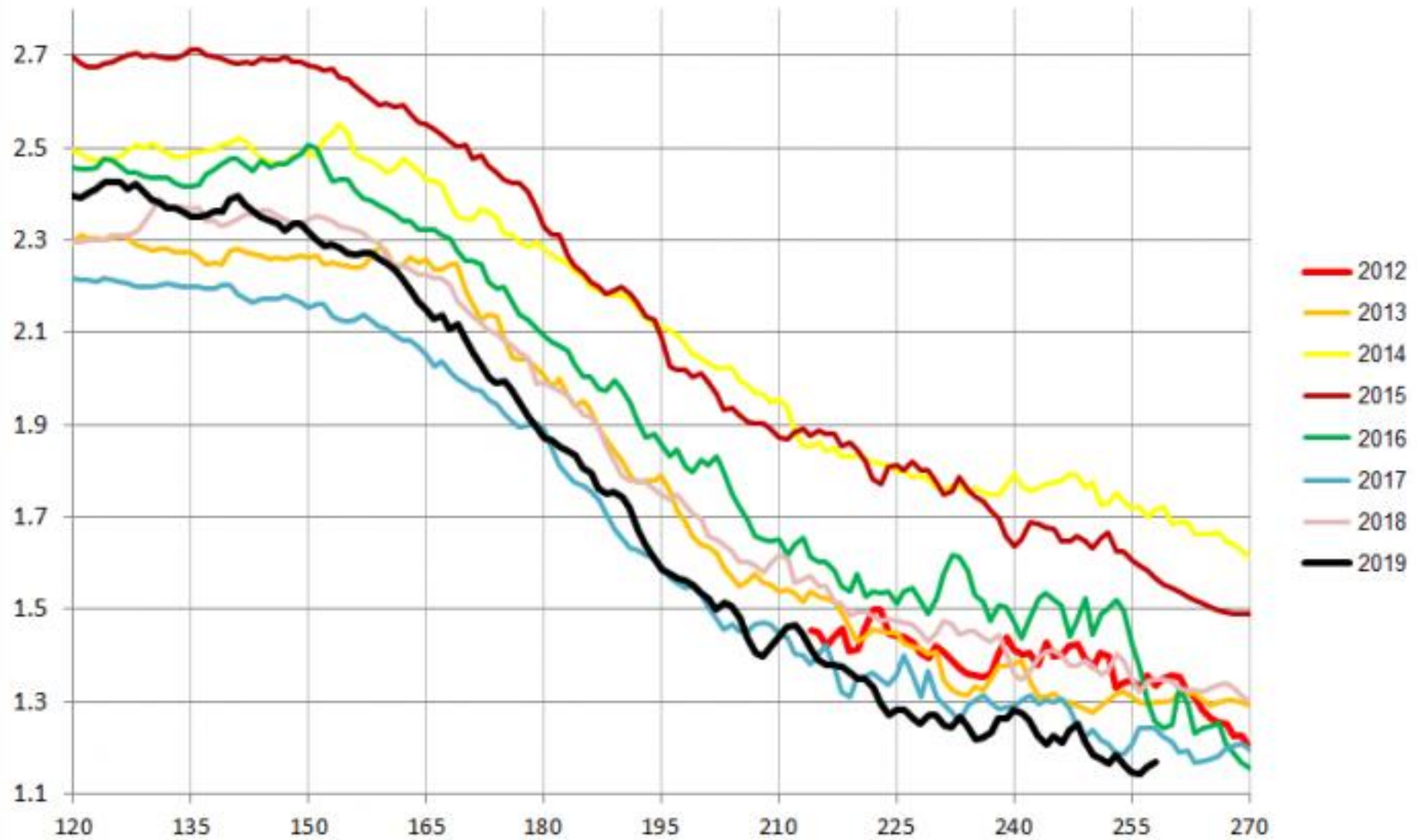
CAB Average Thickness by Year PIOMAS Volume/UH Area
